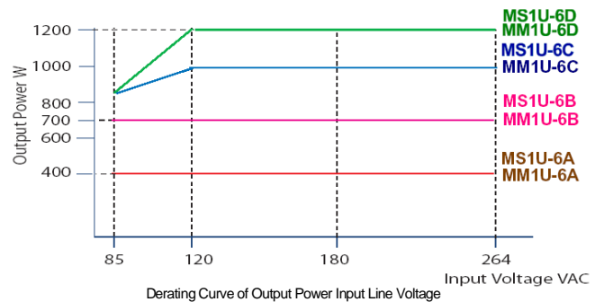
Derating Curve of Output Power Input Line Voltage
