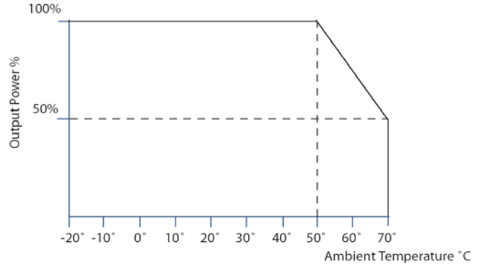
Derating Curve of Output Power versus Ambient Temperature
