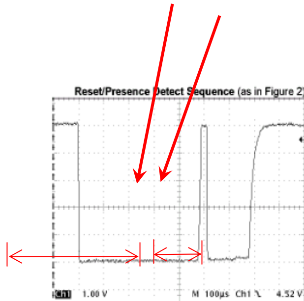
Figure 2a. You can clearly see the negative going reset and the presence pulse
