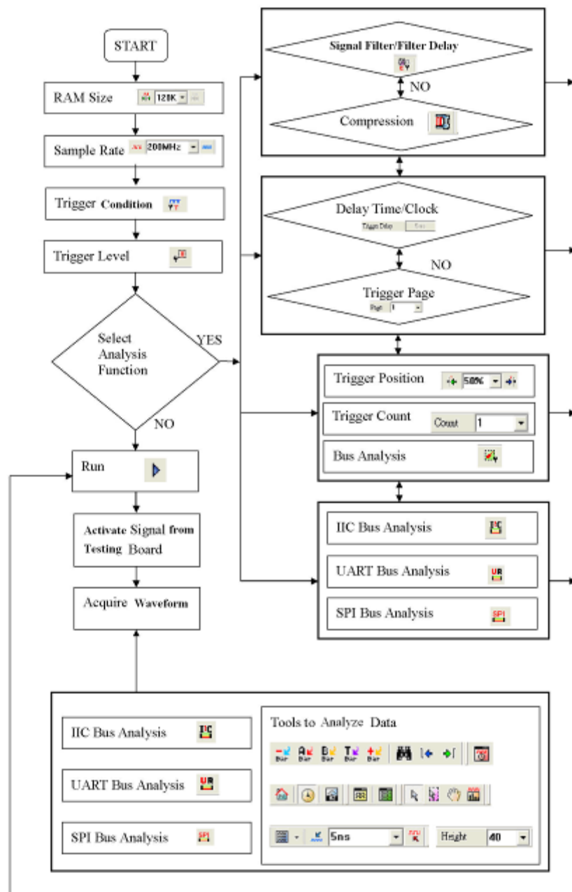
Fig 3-159: Software Flow Diagram
