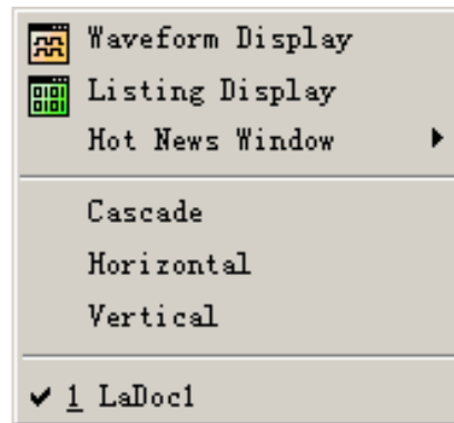
Fig 3-88: Window Menu
