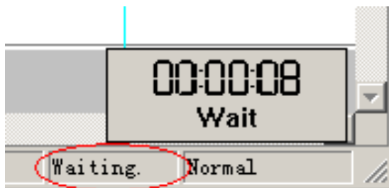
Fig 4-26 – Waiting Status
