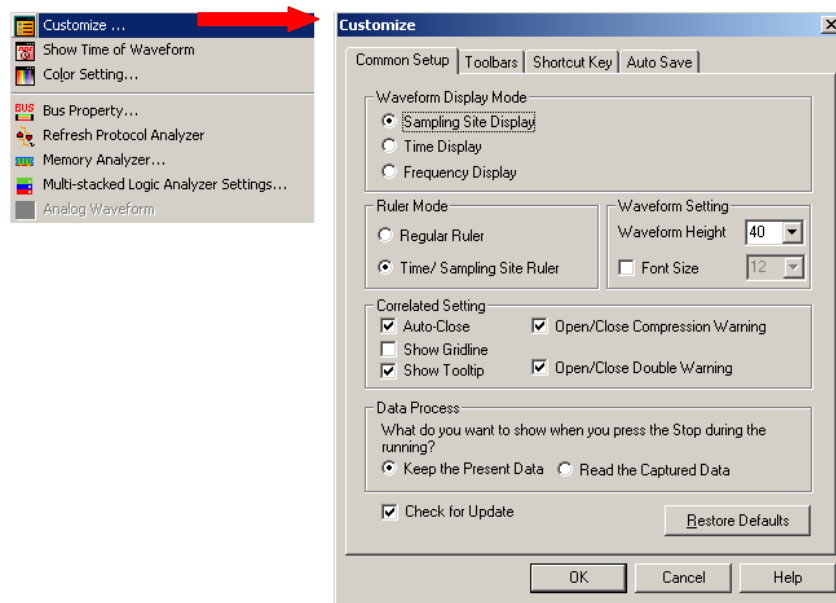
Fig 3-73: Tools Menu
