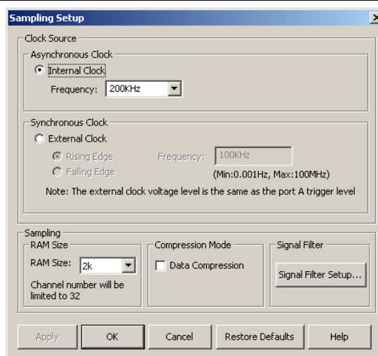
Fig 3-21: Sampling Setup
