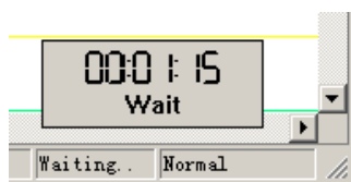
Fig3-99: Stopwatch Function
