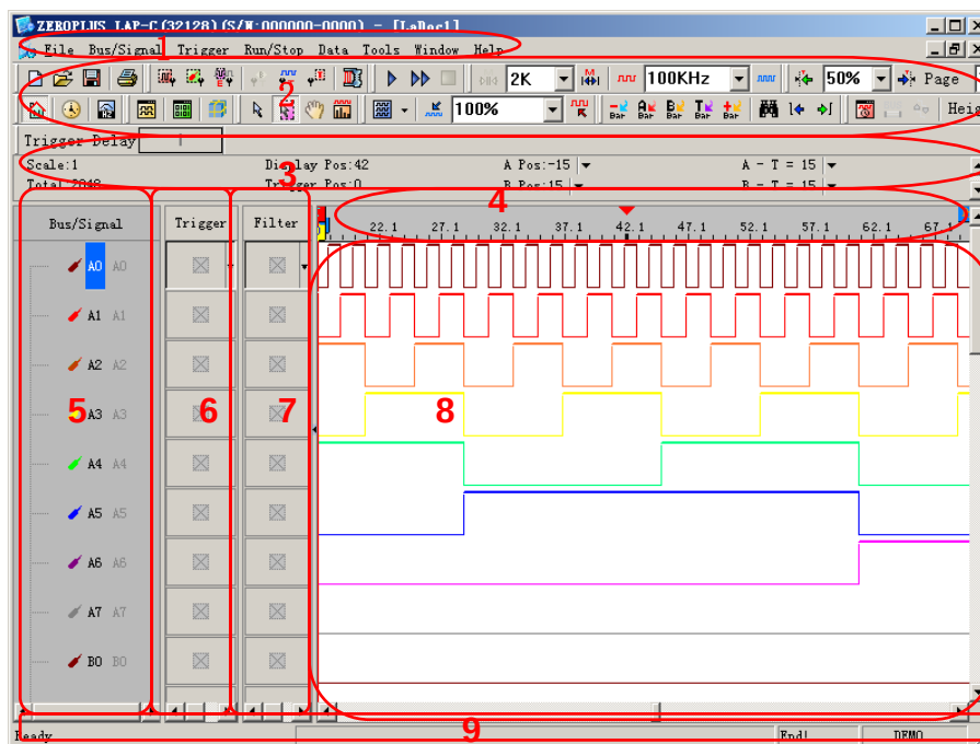
Fig 3-1: Software Interface
