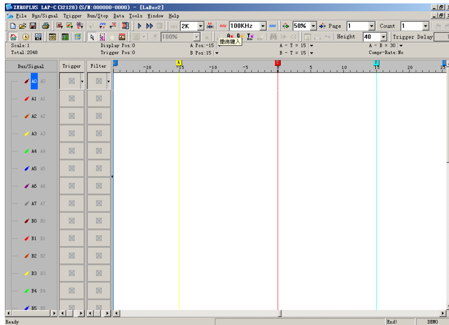
Fig4-130 - User Interface
