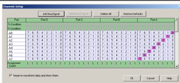
Fig 3-26: Channels Setup
