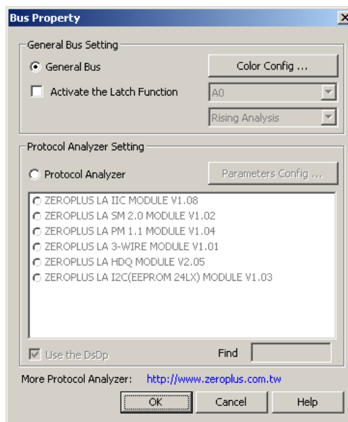
Fig 3-106: Bus Property
