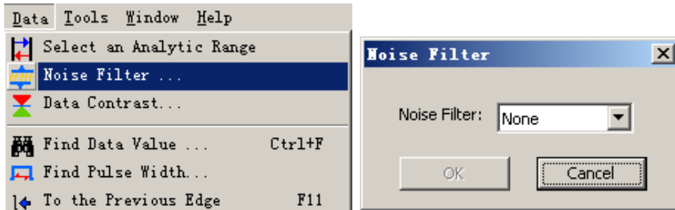
Fig4-150 - Noise Filter
