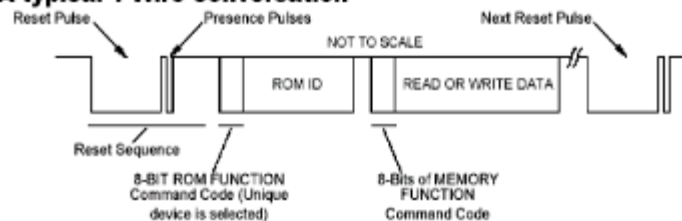
Diagram 1 typical 1-Wire communication sequence.
