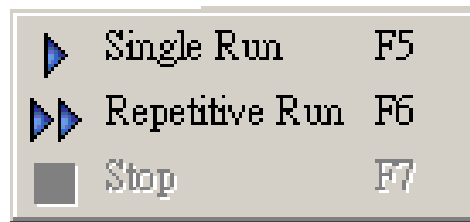
Fig 3-40: Run/Stop Menu
