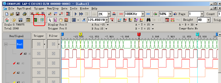
Fig 4-38 - Packet Icon
