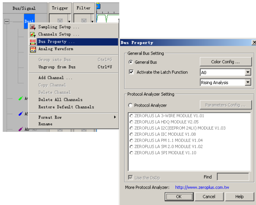
Fig4-66 - Bus Property
