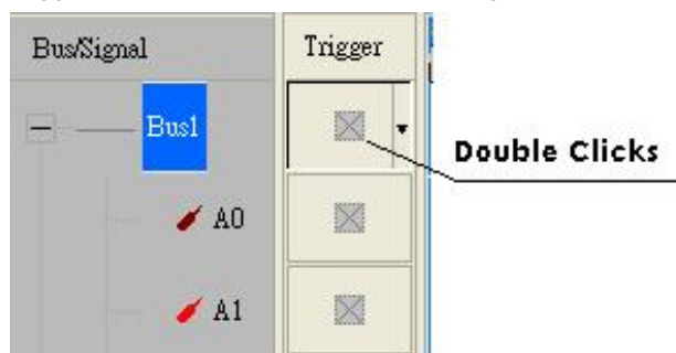
Fig 4-31 – Trigger Column
