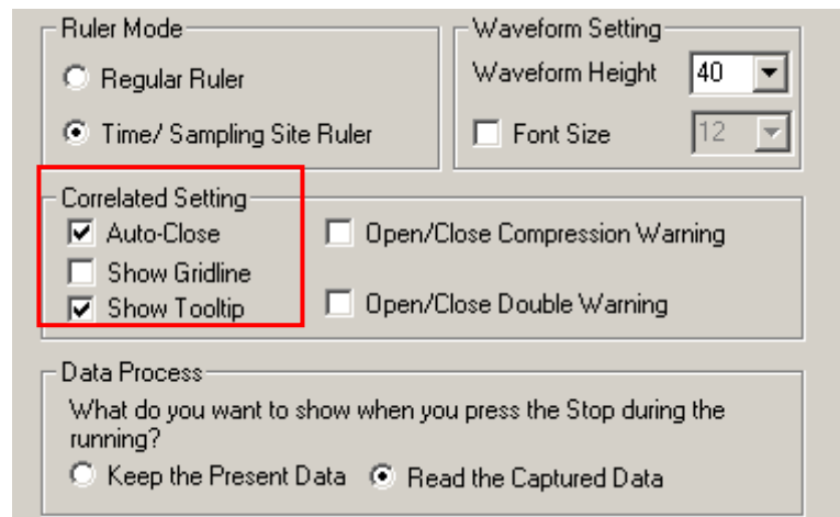
Fig 3-147: Auto-Close
