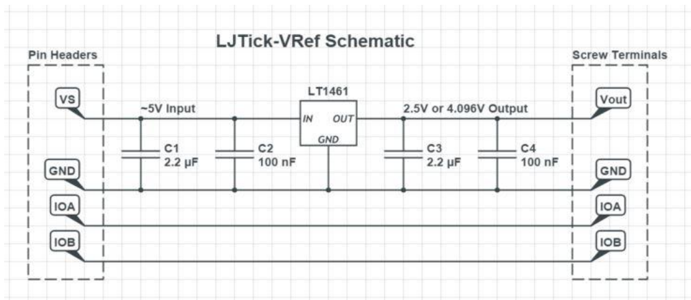
Figure 5: LJTick-VRef Schematic
